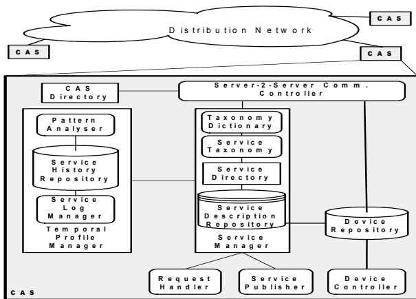
Fig 2: Cell Administration Server (CAS) components
