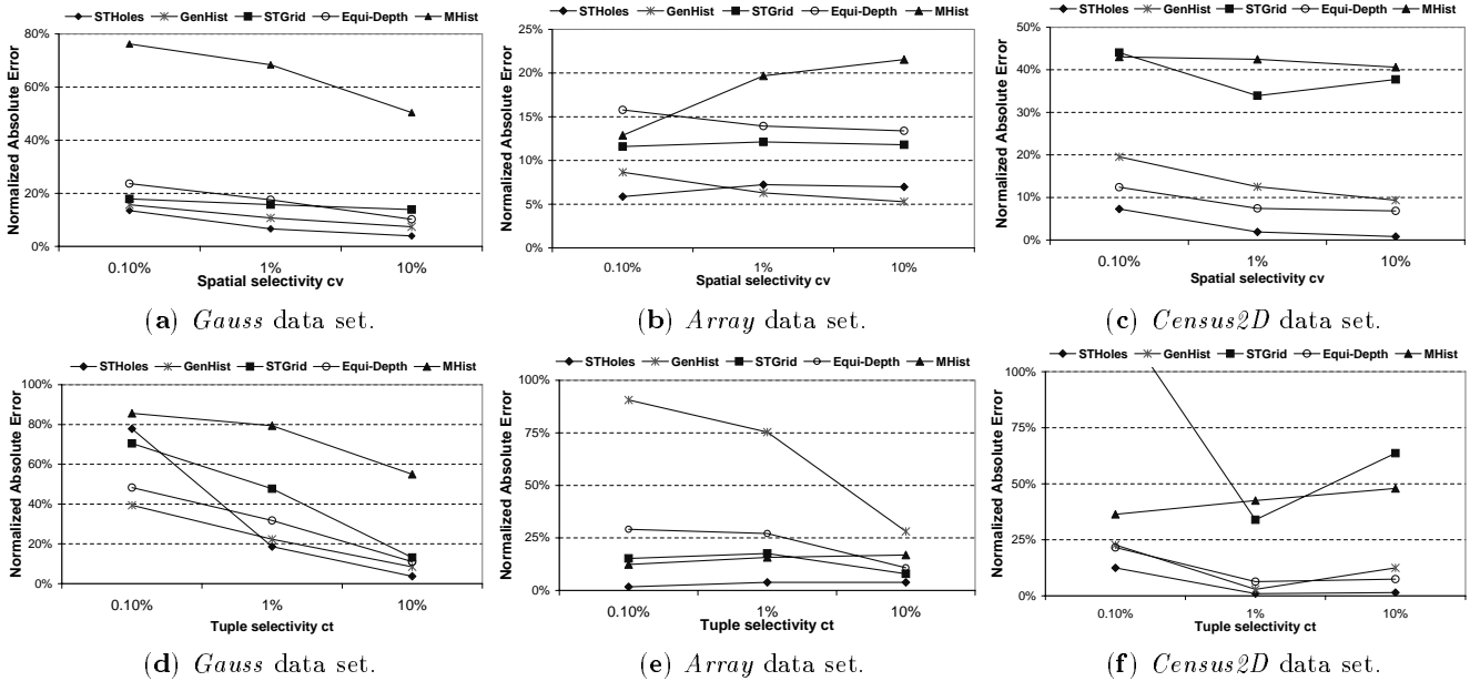
Figure 13: Normalized absolute error using (Data, T[c_t]) for varying spatial ( c_v ) and tuple ( c_t ) selectivity.
