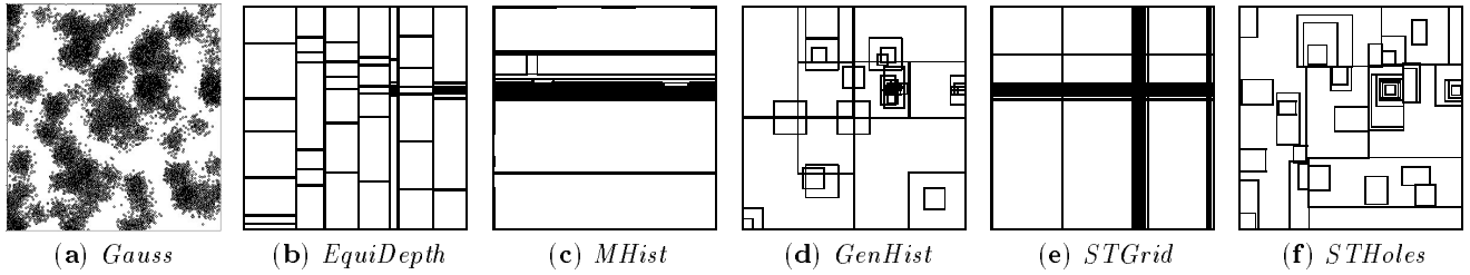
Figure 3: Gauss data set and histograms.
