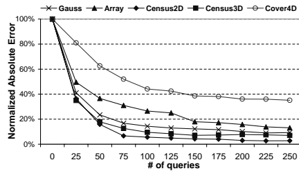
(a) \langle Data, V[1\%] \rangle workload.
