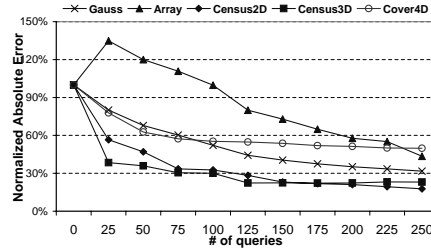
(b) \langle Uniform, V[1\%] \rangle workload.
