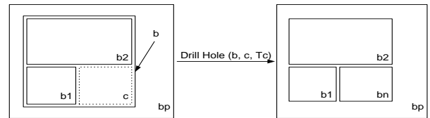
Figure 7: Drilling b_n in bucket b would make b carry no useful information.
