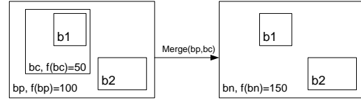
Figure 9: Parent-Child merge.
