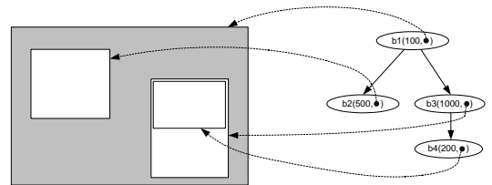
Figure 4: A four-bucket STHoles histogram.
