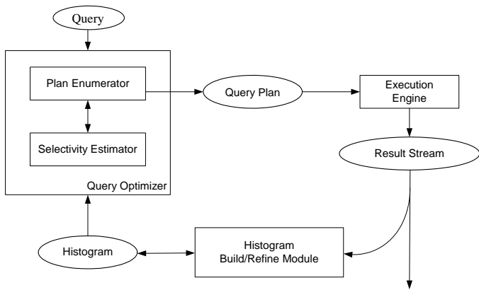
Figure 1: Workload-driven histogram construction.
