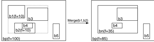
Figure 10: Sibling-Sibling merge.
