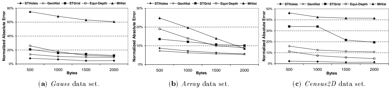
Figure 14: Normalized absolute error for varying histogram sizes.
