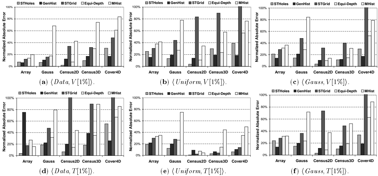
Figure 12: Normalized absolute error for different histograms, data sets and validation workloads.
