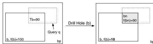
Figure 5: Drilling a hole in bucket b to improve the histogram quality.
