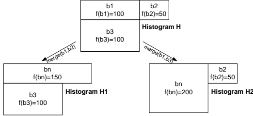
Figure 8: Merging similar buckets.
