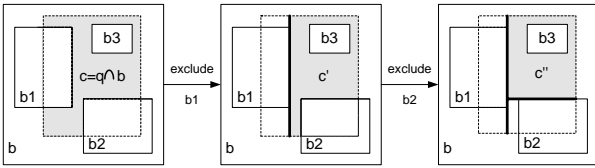
Figure 6: Shrinking a candidate hole c = q \cap b .
