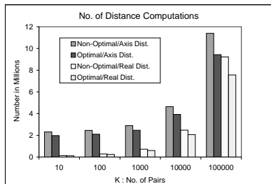
Figure 11: Improvements by Optimized Plane Sweep
