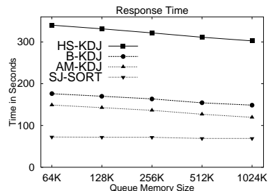
(a) Size of In-Memory Portion of Queue
