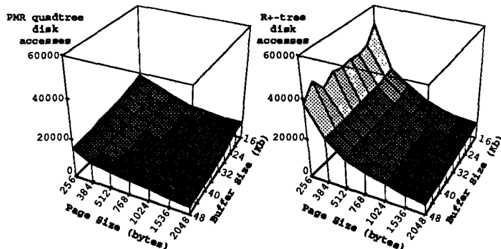
Figure 6: Disk accesses during build by page size and buffer size for the PMR quadtree and the R+-tree.
