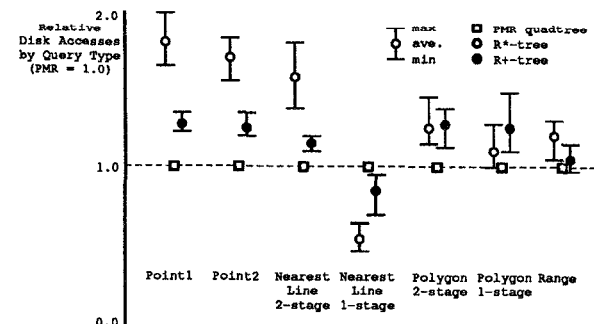
Figure 8: Relative disk accesses.
