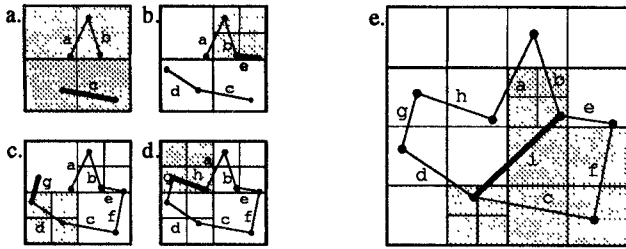
Figure 5: PMR quadtree for the collection of line segments of Figure 1. (a) - (e) illustrate snapshots of the construction process with the final PMR quadtree given in (e).
