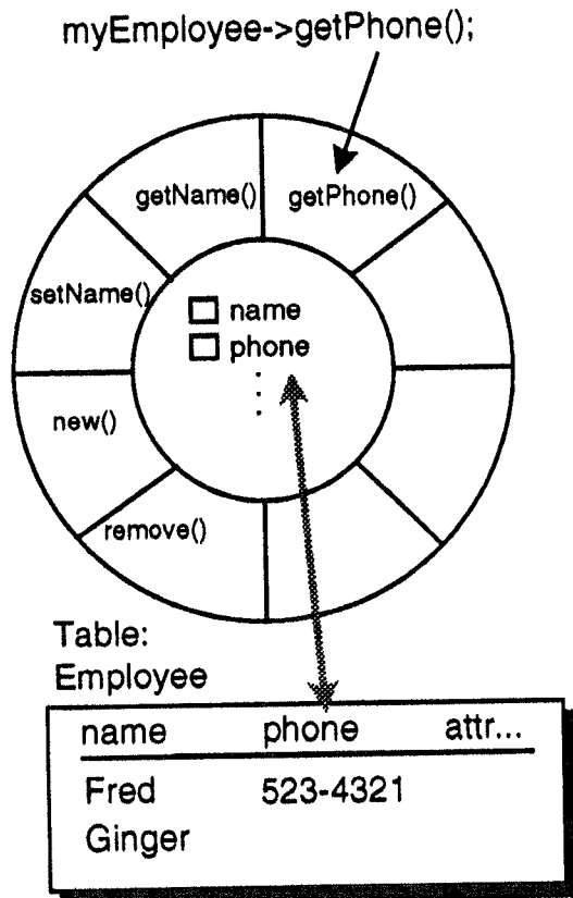
Figure 1. Class definition and mapping.
