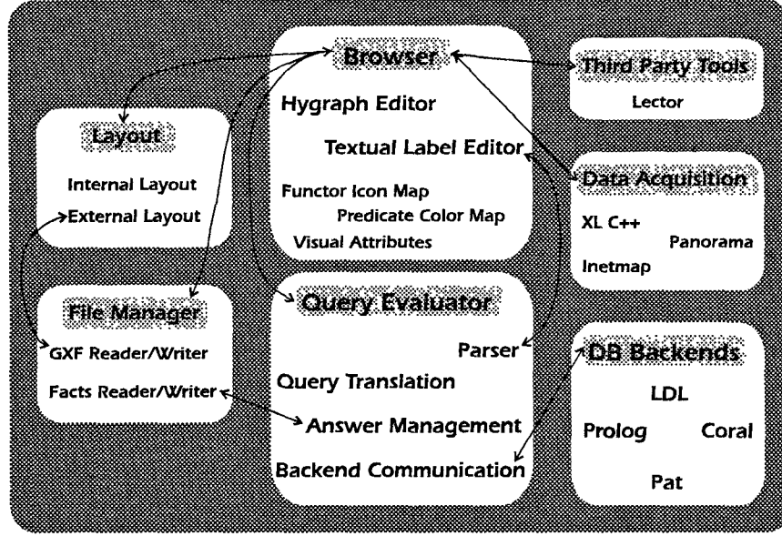
Figure 1: Hy + Architecture Overview.
