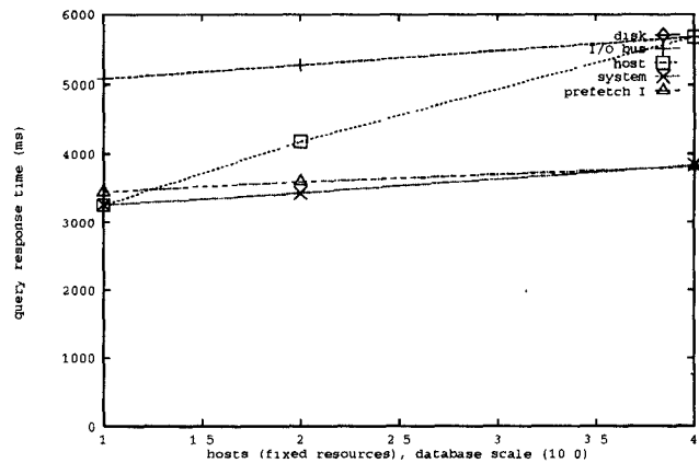
Figure 9: The mainframe vs. workstation trade-off.
