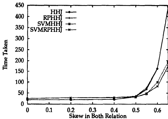
Figure 4: Multi-Bucket Join, Both Relations are Equally Skewed
