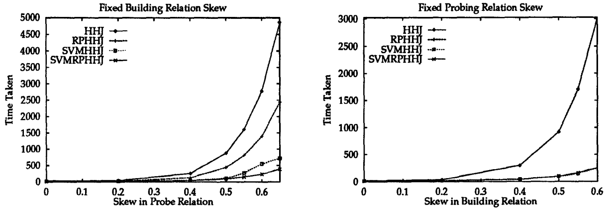
Figure 3: Double Skew, One Relation skewed at 1 - \theta = 0.9
