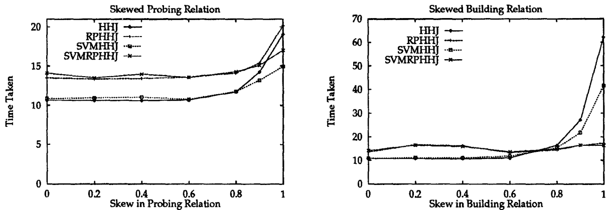
Figure 1: Single Relation Skew
