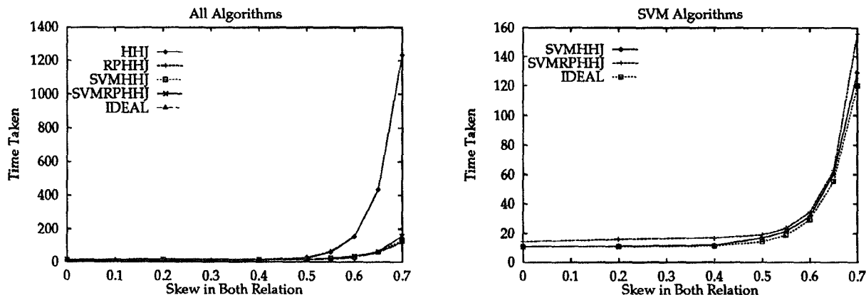
Figure 2: Join Product Skew, Both Relations are Equally Skewed
