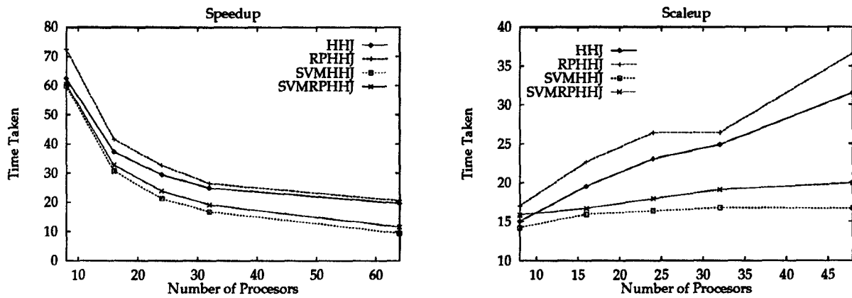
Figure 3: Double Skew, One Relation skewed at 1 - \theta = 0.9
