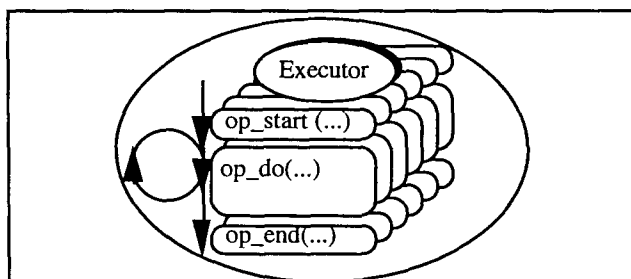
Figure 13: The flow within an executor process is to call the op_start() entry of each operator belonging. Then the executor calls any op_do() operation that has an input buffer. When all operations return a completion code, the executor calls op_end() for all operations and then terminates the process. Each op_do() step processes one or more input buffers and passes them downstream to the next river and operators.
