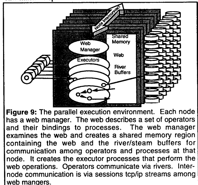
Figure 9: The parallel execution environment. Each node has a web manager. The web describes a set of operators and their bindings to processes. The web manager examines the web and creates a shared memory region containing the web and the river/steam buffers for communication among operators and processes at that node. It creates the executor processes that perform the web operations. Operators communicate via rivers. Inter-node communication is via sessions tcp/ip streams among web managers.
