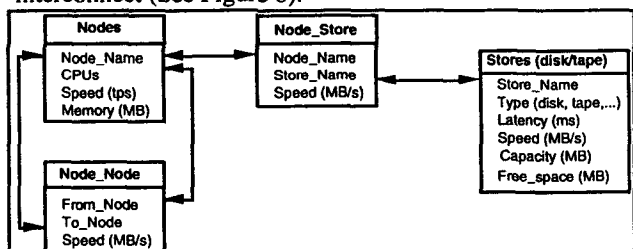
Figure 6: The entity-relationship diagram of the cluster configuration database built by the explorers executing at each node. The Nodes table describes the processors and memory at each node. The Stores table describes the speed, capacity, and free space of each disk and tape robot. The Node_Store and Node_Node tables record the point-to-point connectivity and bandwidth between directly-connected nodes and disks and among nodes.
