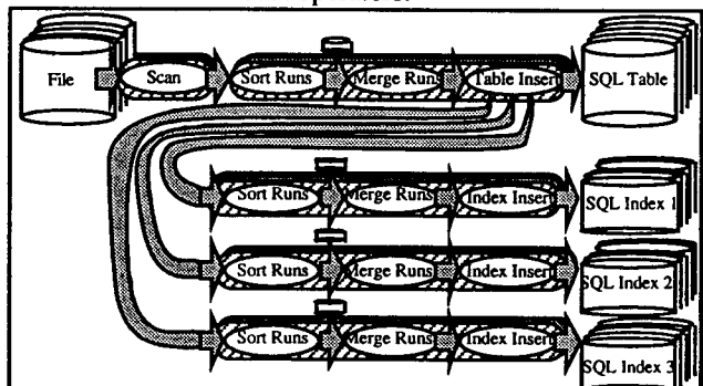
Figure 8: The template for a load plan showing operator-process bindings, rivers, and showing a two-pass sort. Each index build is done by a separate group of processes. This template also shows possible partition parallelism.
