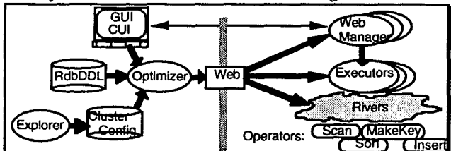
Figure 5: The parallelism prototype has a planning phase shown at the left and an execution phase at the right. The optimizer generates a parallel plan (web) based on the job definition, the database definition, and the cluster configuration. The client starts the plan execution by forking a web-manager. It in turn forks web managers in each other cluster node. The web managers fork executors at their nodes. The executors perform their part of the web by creating a thread per operator. The operators communicate via the river system.
