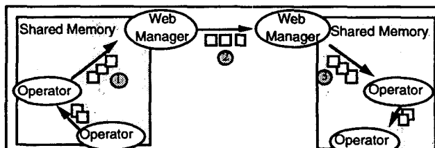
Figure 11: The three-hop message protocol used by MIO-SIO to reduce the polynomial explosion. LAN streams and rivers travel via MIO (1) to the local web manager that then multiplexes them over a tcp/ip sessions SIO (2) to other web managers. MIO is used at the destination to deliver the data to the destination operator. Since MIO is a zero-copy message protocol, it adds less than 10% to the message cost. A three-level multiplexing scheme would be needed for clusters much larger than 100 nodes (600 processors).
