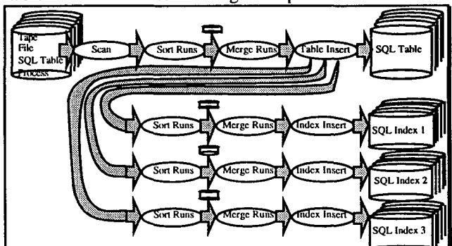
Figure 4: The dataflow graph of a single-table database load operation. Input records must be sorted by the clustering key in order to build the base table -- otherwise the insert operation would do random disk IO and would run 100-times slower. The base table has three secondary indices in this example. The index records are of the form: (alternate-key, record_id). One cannot construct the index record until the base table record has been placed and its record_id assigned by the database system. The table insert operator builds these index records. Each index load has a dataflow graph similar to table-load graph. If the base table or indices are hashed, then a hash operator (MakeDBkey) must be inserted prior to the sort step in the flow, so that records can be sorted in hash order. Each node of the graph can be cloned for partition parallelism.
