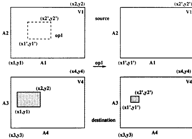
Figure 5: Effect of op_1 in the Presence of a Cursor
