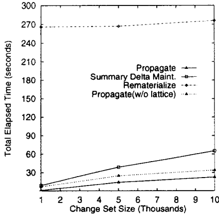
(a) Varying change size for update-generating changes
