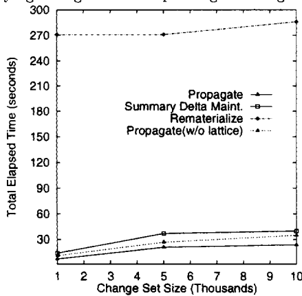
(c) Varying change size for insertion-generating changes
