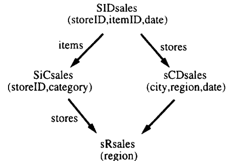
Figure 8: The \mathcal{V} -lattice for the retail warehousing example
