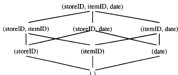
Figure 4: Data Cube Lattice.
