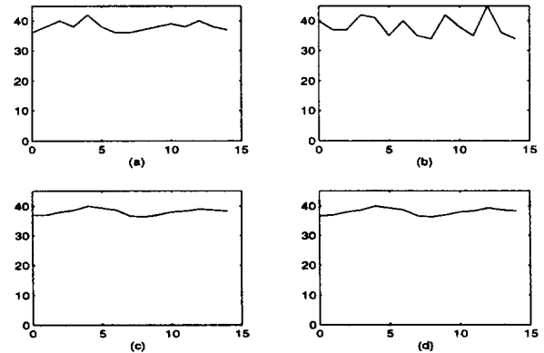
Figure 1: (a) Time sequence \vec{s}_1 = (36, 38, 40, 38, 42, 38, 36, 36, 37, 38, 39, 38, 40, 38, 37) , (b) time sequence \vec{s}_2 = (40, 37, 37, 42, 41, 35, 40, 35, 34, 42, 38, 35, 45, 36, 34) , (c) the 3-day moving average of \vec{s}_1 , and (d) the 3-day moving average of \vec{s}_2
