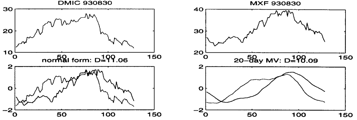
Figure 5: From left to right, top to bottom: the daily closing price of Digital Microwave Corp. ( DMIC ) starting from “93/08/30” for 128 days, the daily closing price of The Mexico Fund Inc. ( MXF ) for the same period, their normal forms, and the 20-day moving averages of both series (D denotes the Euclidean distance)
