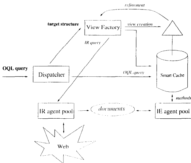
Figure 2: AKIRA’s architecture.
