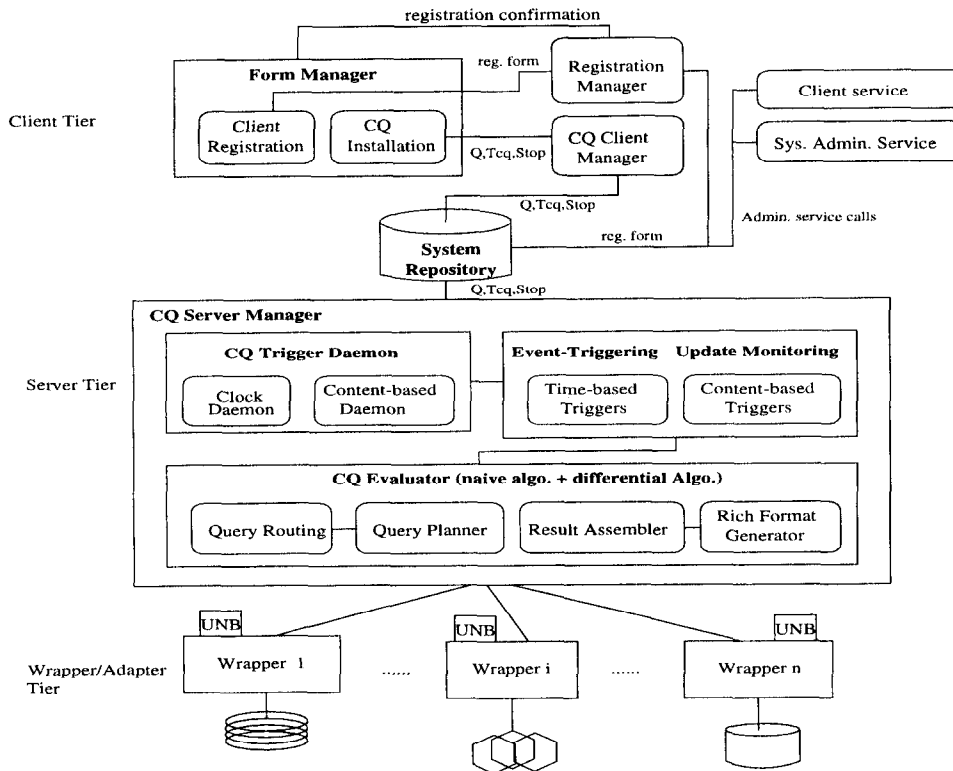
Figure 1: System architecture
