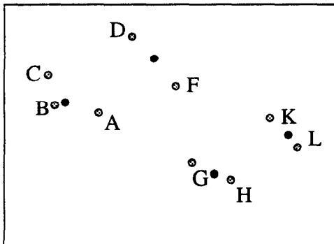
(b) Approximate-SVD
