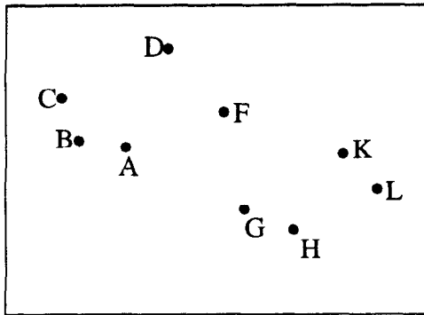
(a) All-Data-SVD
