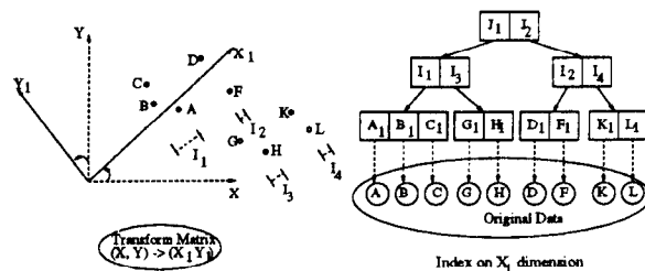
Figure 8: Index structure after adding 4 new data items G, H, K and L .
