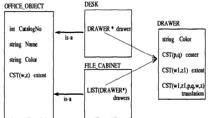
Figure 1: A Constraint Object-Oriented Database Schema
