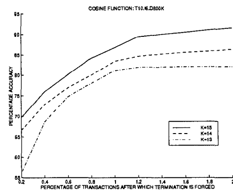
Figure 13: Percentage accuracy scaling with different levels of early termination (cosine)
