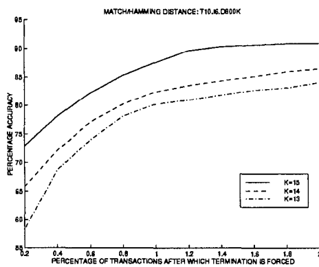
Figure 10: Percentage accuracy scaling with different levels of early termination (match/hamming distance)
