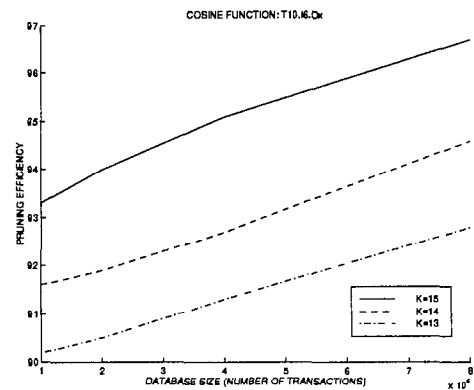
Figure 12: Scaling of pruning performance with database size (cosine)
