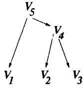
Figure 3: Example VDAG
