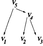
Figure 6: VDAG
