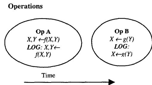
Figure 5: An example showing that a more precise flush order is possible than what is captured in W .
