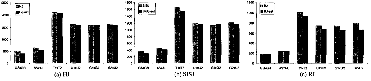
Figure 10: Experimental and analytically estimated page accesses for the various joins
