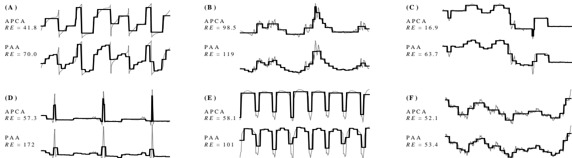
Figure 4: A comparison of the reconstruction errors of the equal-size segment approach (PAA) and the variable length segment approach (APCA), on a collection of miscellaneous datasets. A) INTERBALL Plasma processes. B) Darwin sea level pressures. C) Space Shuttle telemetry. D) Electrocardiogram. E) Manufacturing. F) Exchange rate.
