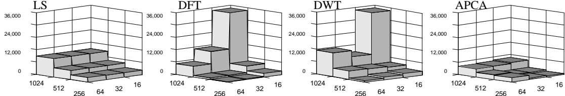
Figure 12: Comparison of LS, DFT, DWT and APCA techniques in terms of I/O cost (number of random disk accesses). For LS, the cost is computed as number_sequential_disk_accesses/10 .
