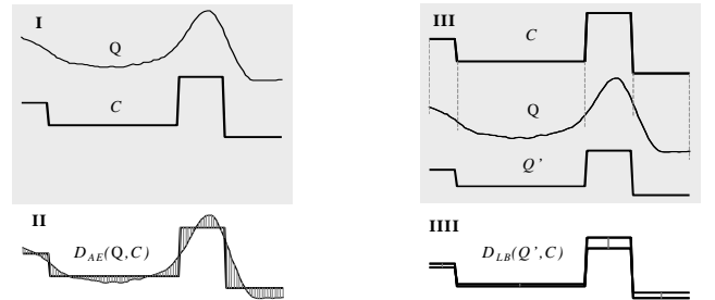
Figure 6: A visualization of the two distance measures defined on the APCA representation. I) A query time series Q and an APCA object C . II) The D_{AE} measure can be visualized as the Euclidean distance between Q and the reconstruction of C . III) Q' is obtained by projecting the endpoints of C onto Q and calculating the mean values of the sections falling within the projected lines. IIII) The D_{LB} measure can be visualized as the square root of the sum of the product of squared length of the gray lines with the length of the segments they join.
