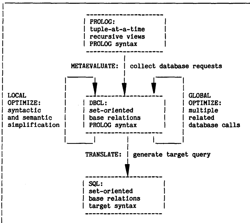
Figure 1: Architecture of PROLOG-SQL translation mechanism
