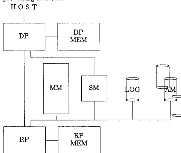
Figure 1 MMDB Model
