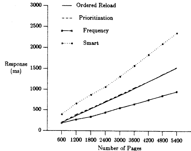
Figure 5. Effect of Number of Pages on Transaction Response Time
