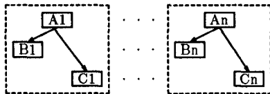
Figure 10. Intra-Object Clustering
