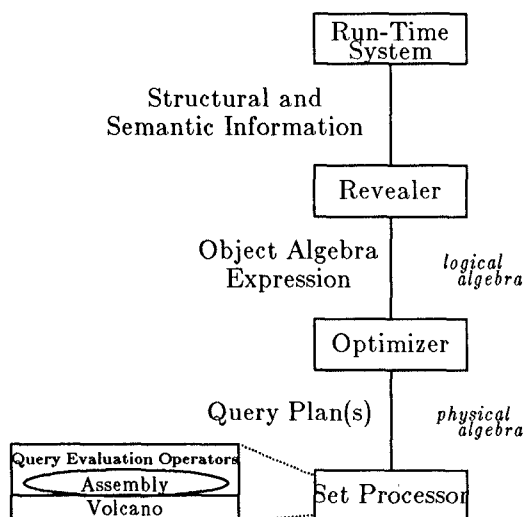
Figure 1. Revelation Architecture
