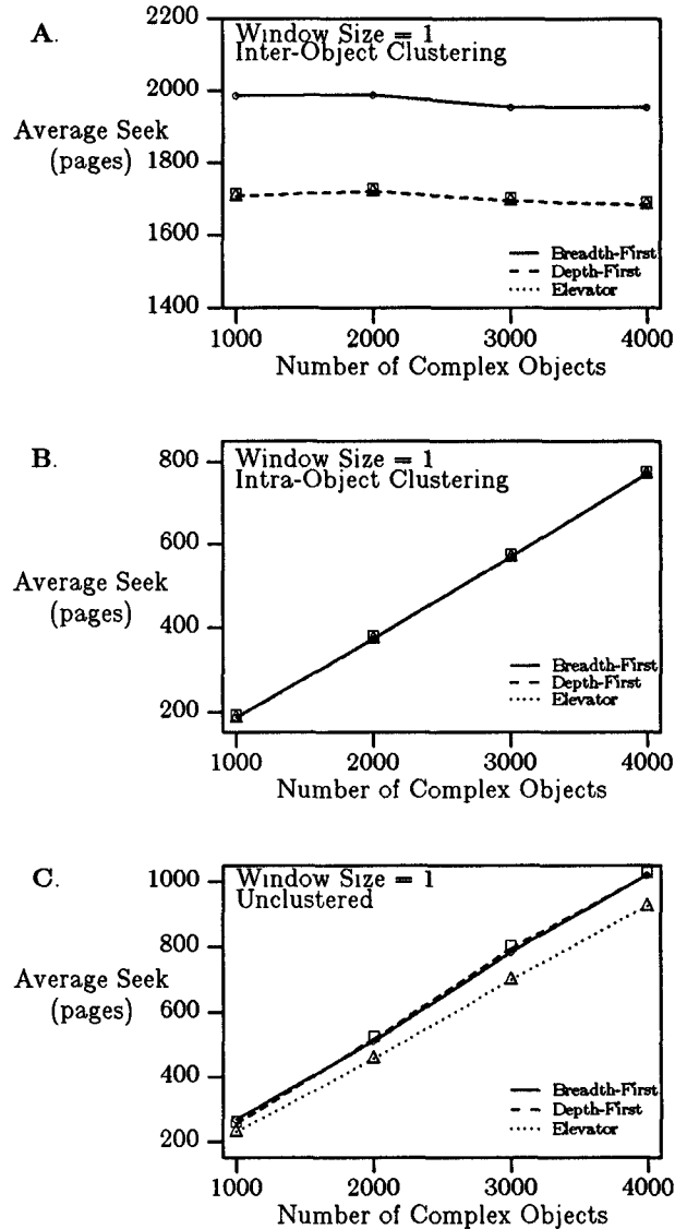
Figure 11. Scheduling Algorithm vs. Database Size (Window Size = 1)
