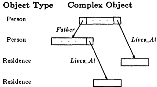
Figure 2. Sample Complex Object
