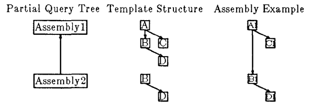
Figure 17. Bottom-up and Top-down Assembly
