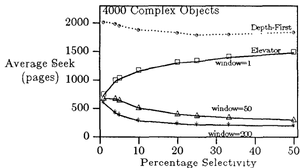
Figure 16. Predicates and Selectivities
