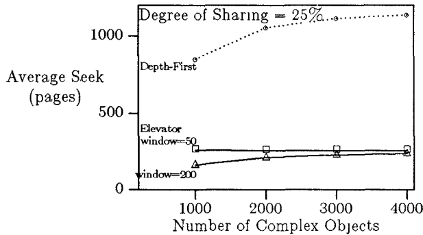
Figure 15. Performance with Shared Objects
