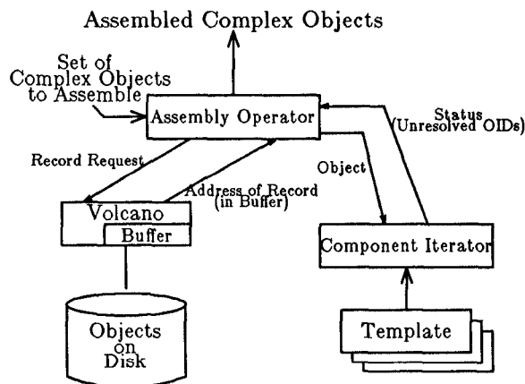
Figure 6. Assembly Operator Architecture
