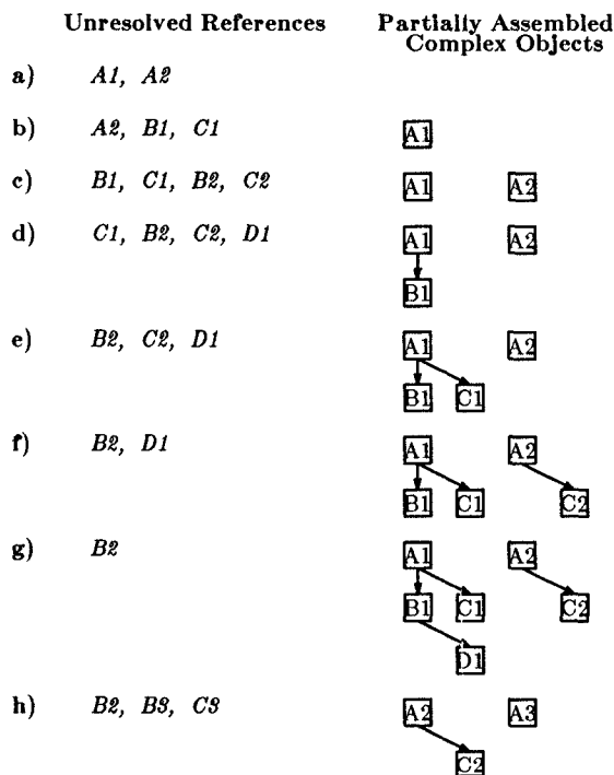
Figure 5. Sliding Assembly Operator Example
