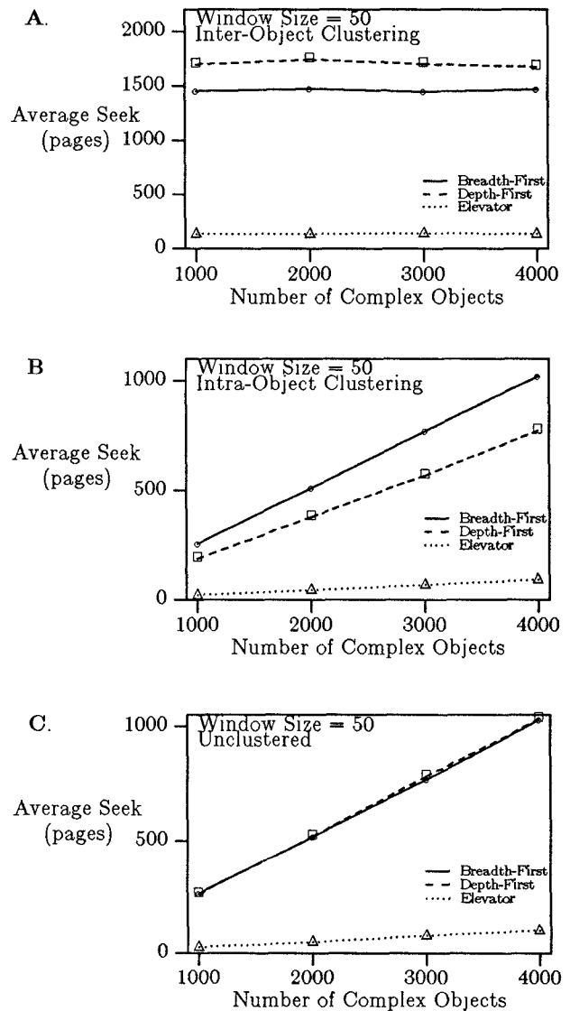
Figure 13. Scheduling Algorithm vs. Database Size (Window Size = 50)
