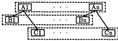
Figure 9. Inter-Object Clustering
